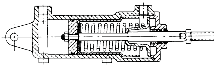
ASSEMBLY VIEW
