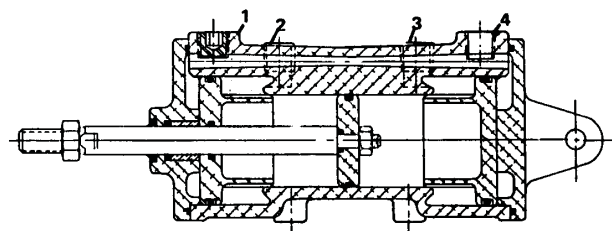
Assembly View
