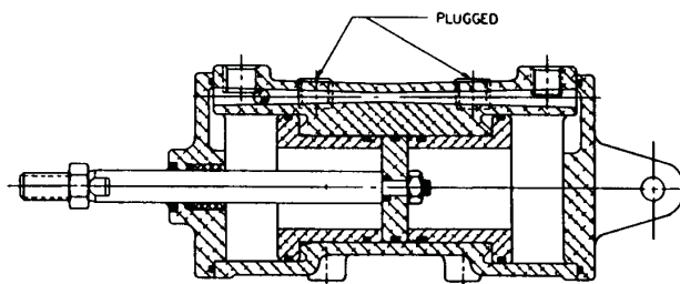
Assembly View
