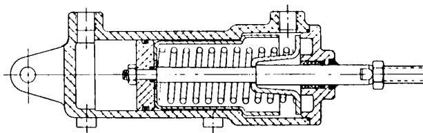
Assembly View
