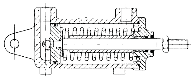
Assembly View (Single-Acting Model)
